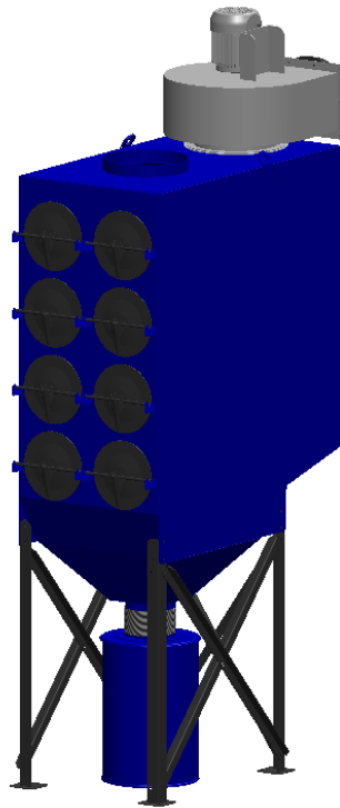
DCF1680 8000cfm@12" SP 15hp Blower
